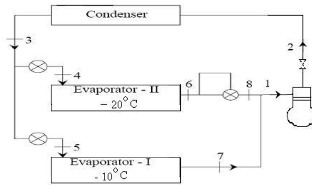
Fig.17.3: Two evaporators operating at different temperature and one compressor system
