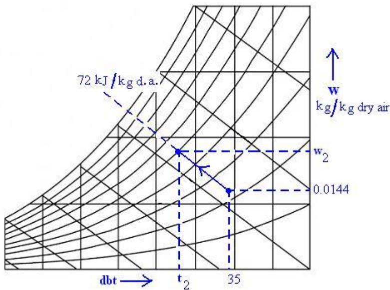
Fig 29.6: Psychrometric chart
