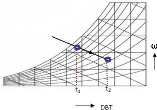
Fig.27.7: Adiabatic dehumidification
