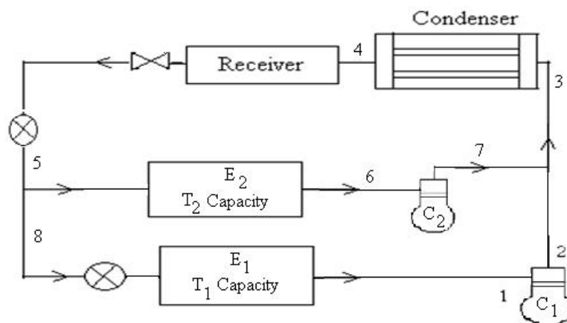
Fig.20.1: Multievacuator and individual compressor system
