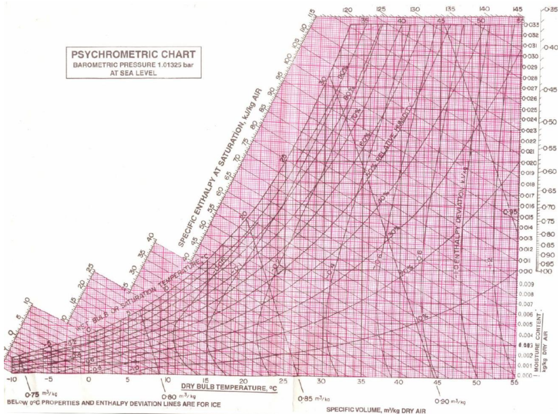
Fig. 26.3 Psychrometric chart
